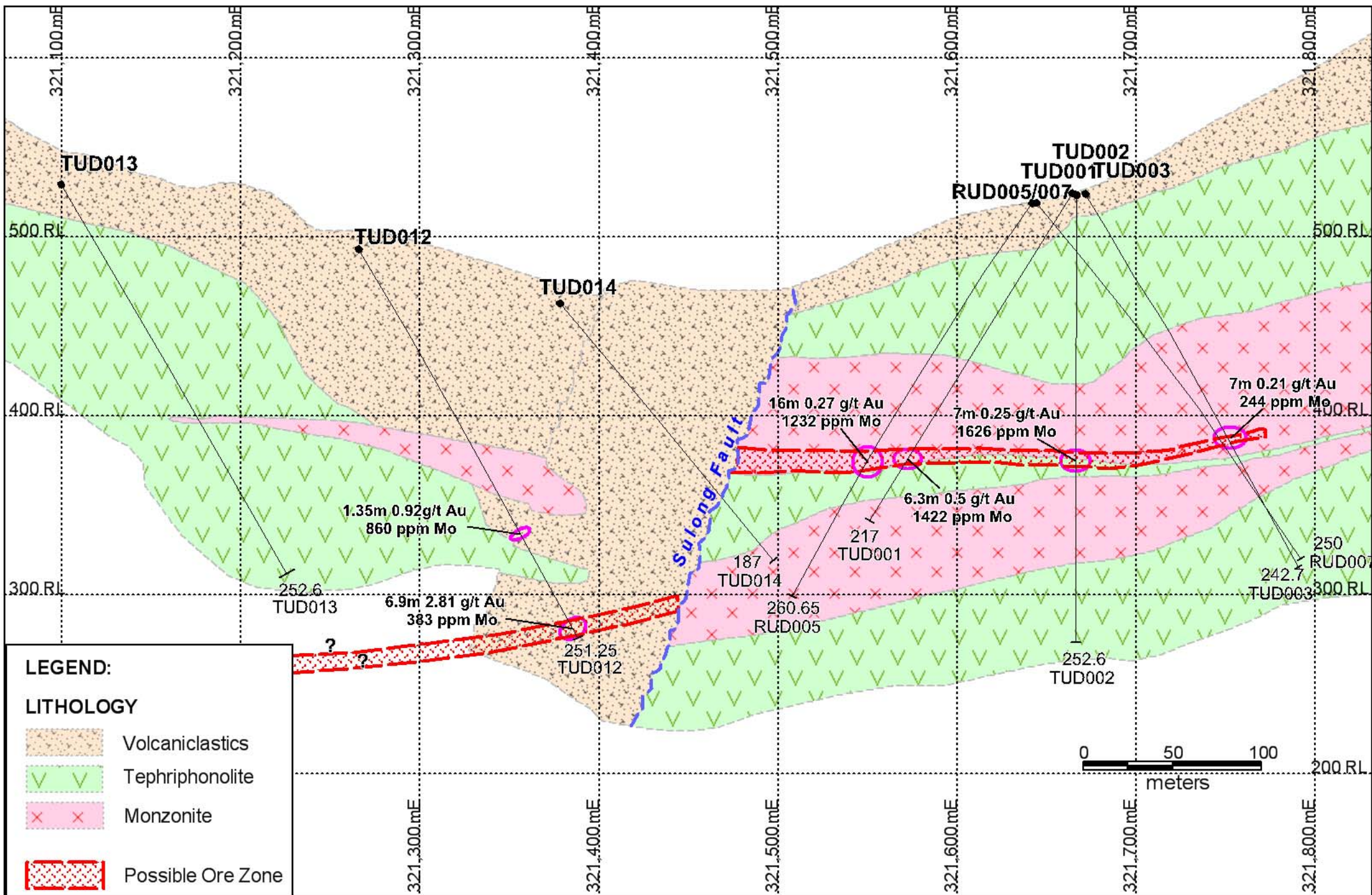
Schematic Cross Section Along 1,814,000N - Looking North Tulingan Au Prospect
