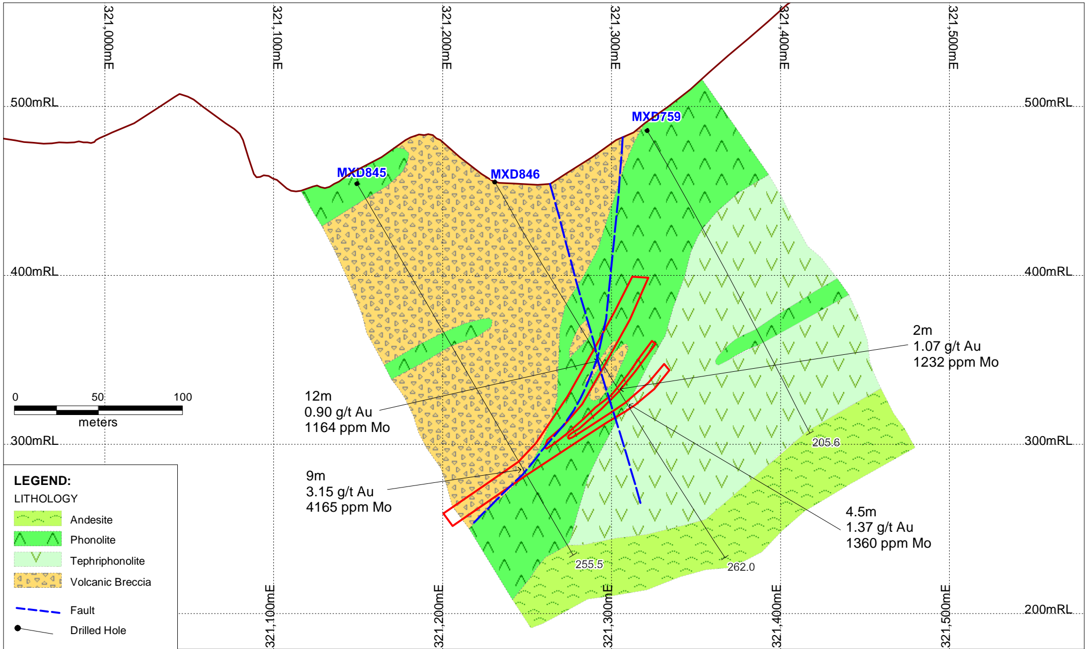
Schematic Cross Section Along L1814250N Looking North Malilibeg South
