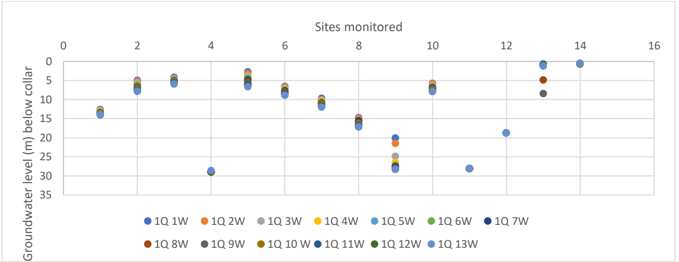
Weekly groundwater level for the 14 piezometers located in the TSF and La Simona area, data from the 1Q 2021 is shown below:
