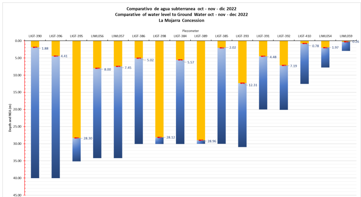
Figure 4.2.2.1 a. Behavior of groundwater levels in La Mojarra concession.
