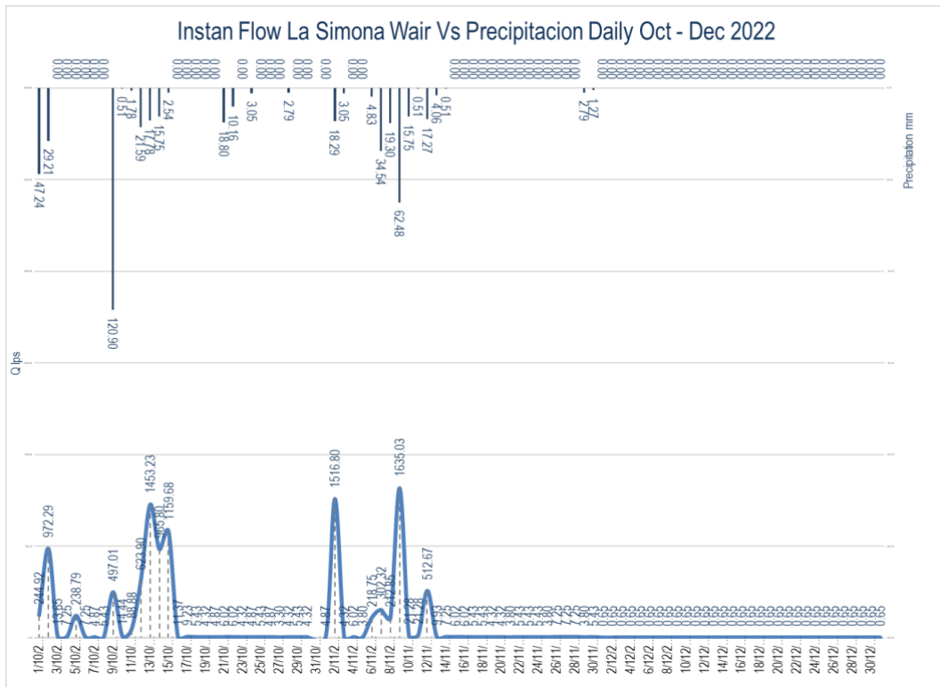
Figure 3.6.1.1 a. Behavior of flows vs precipitation La Simona weir.
