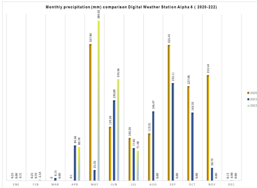
Figure 4.9.1.3 a. Historical data of the Digital Station CONDOR S.A – 2020 – 2022
