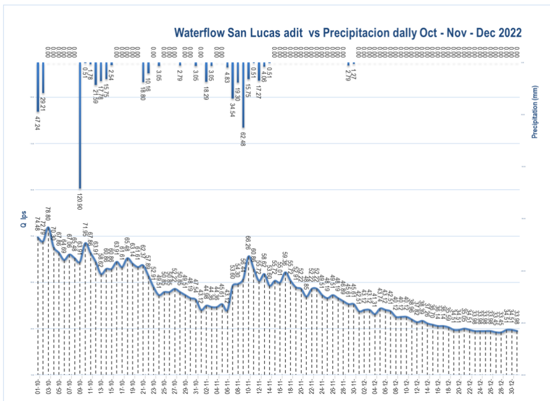
Figure 3.6.1.1 a. Behavior of flows vs precipitation in San Lucas Tunnel - Ocotillo.
