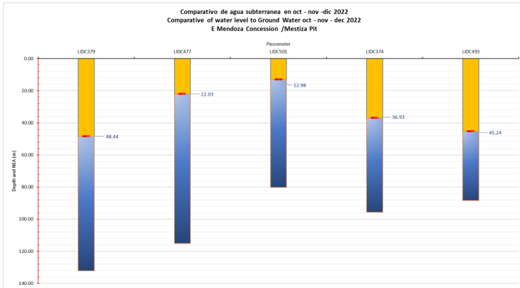
Figure 5.2.1.2 a. Behavior of groundwater levels in Espinito Mendoza concession.
